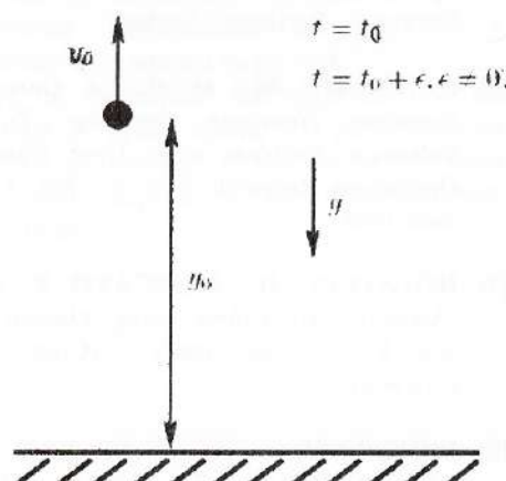
FIGURE 1 A short introduction to dynamical systems Two-body system
