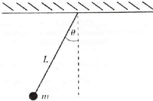
FIGURE 3 A short introduction to dynamical systems Simple pendulum
